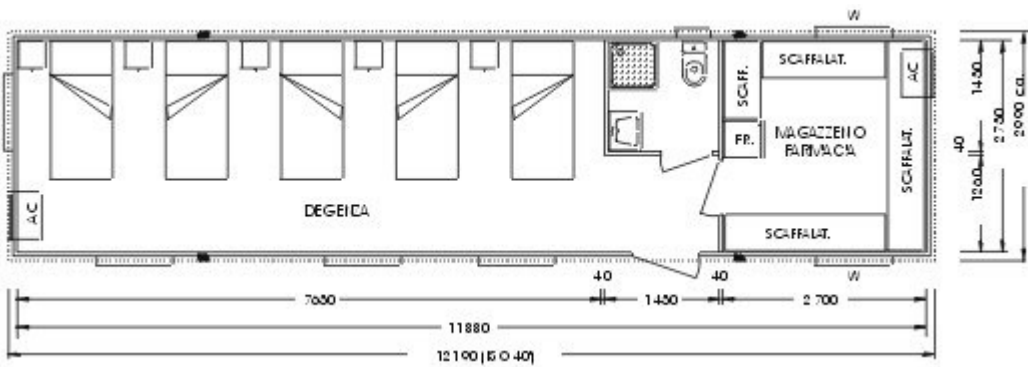
Modulo day - hospital
